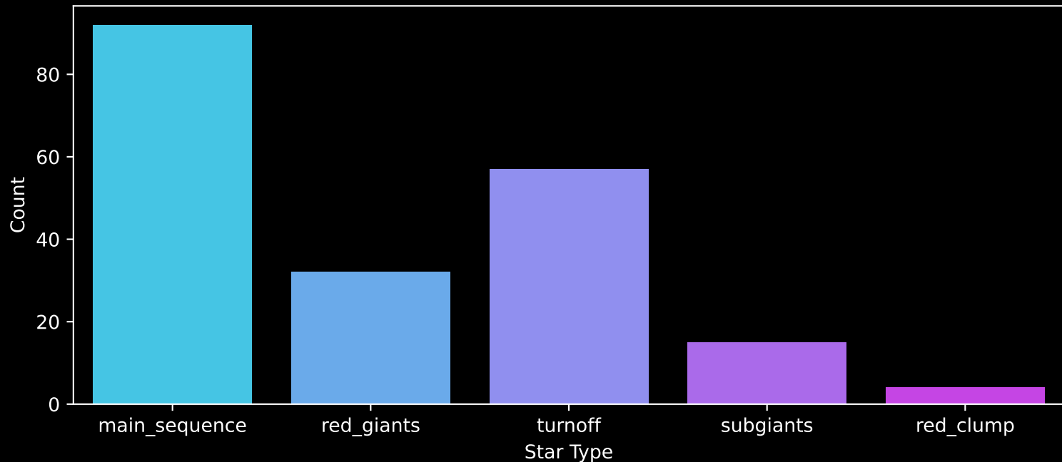
APOGEE DR17 Field: [K2_C12_077-57_btx] Count plot of Star Type
