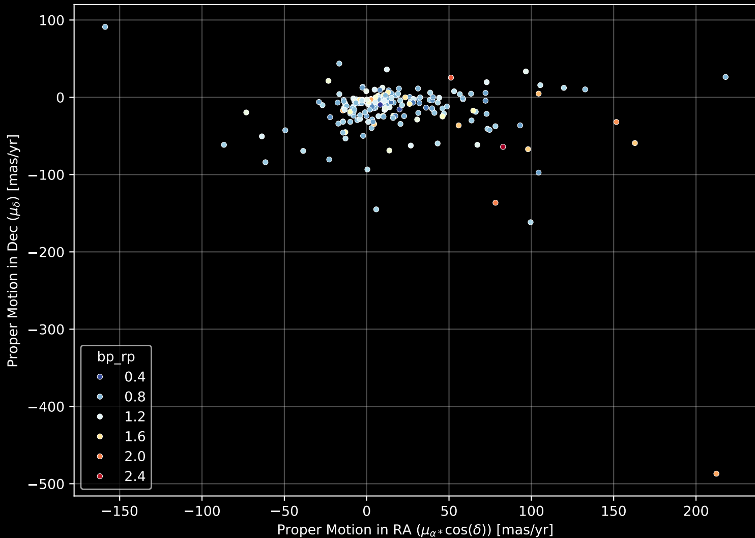
APOGEE DR17 Field: [K2_C12_077-57_btx] Proper Motion Diagram (n= 200)
