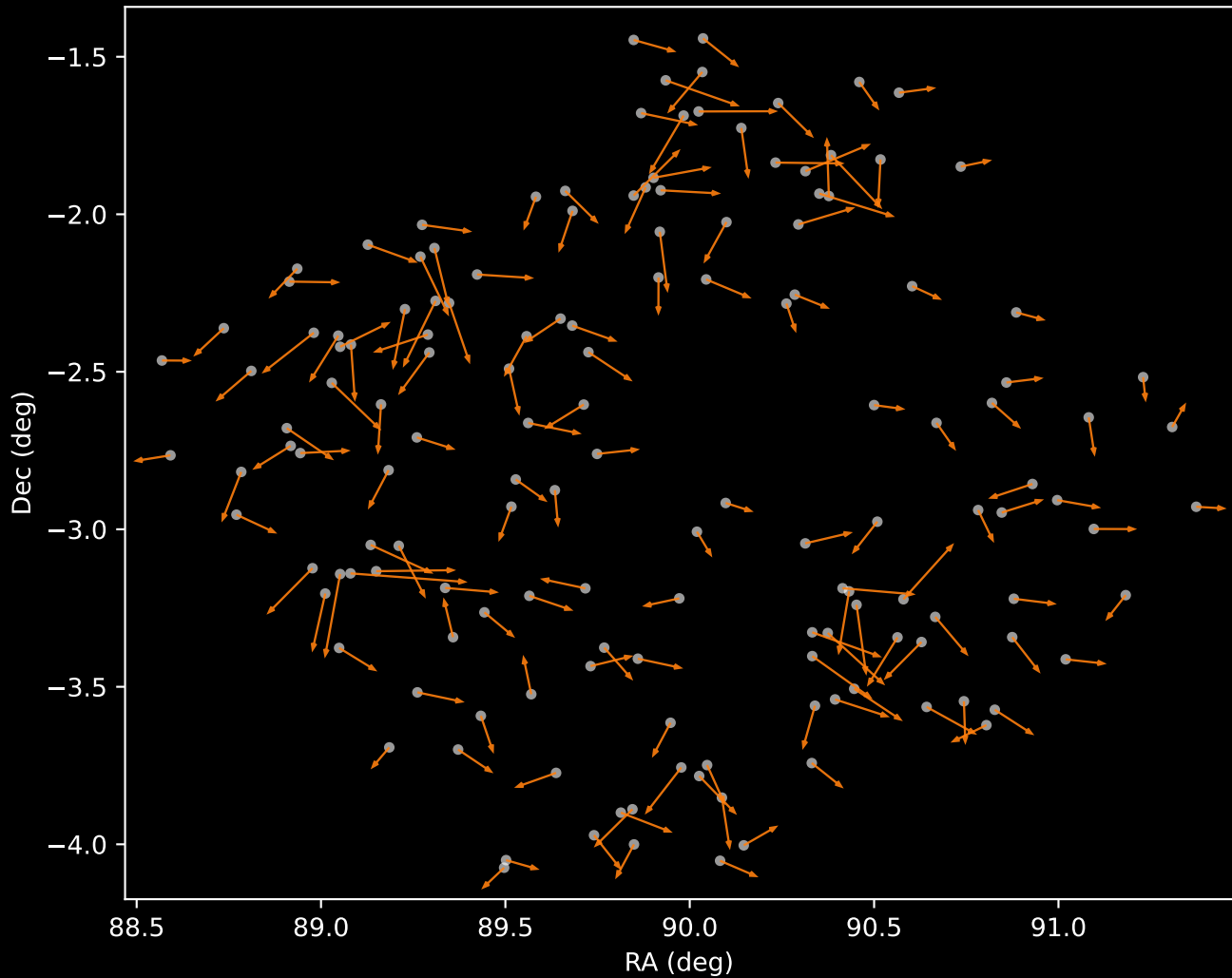
APOGEE DR17 Cluster 2 Proper Motion Vectors (n=149)
