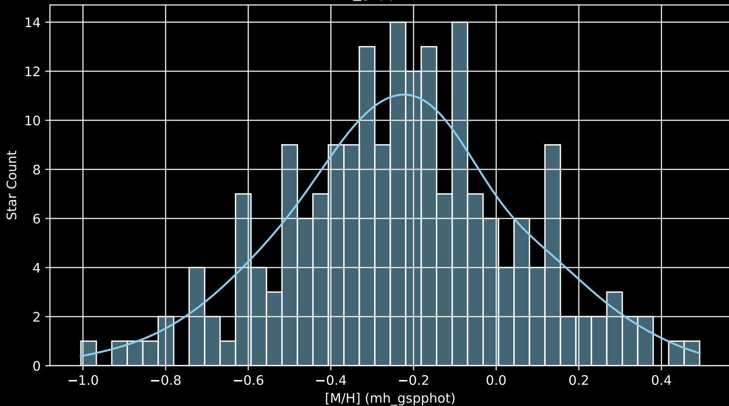
APOGEE DR17 Field: [K2_C12_077-57_btx [M/H] (mh_gspphot) (n= 200)
