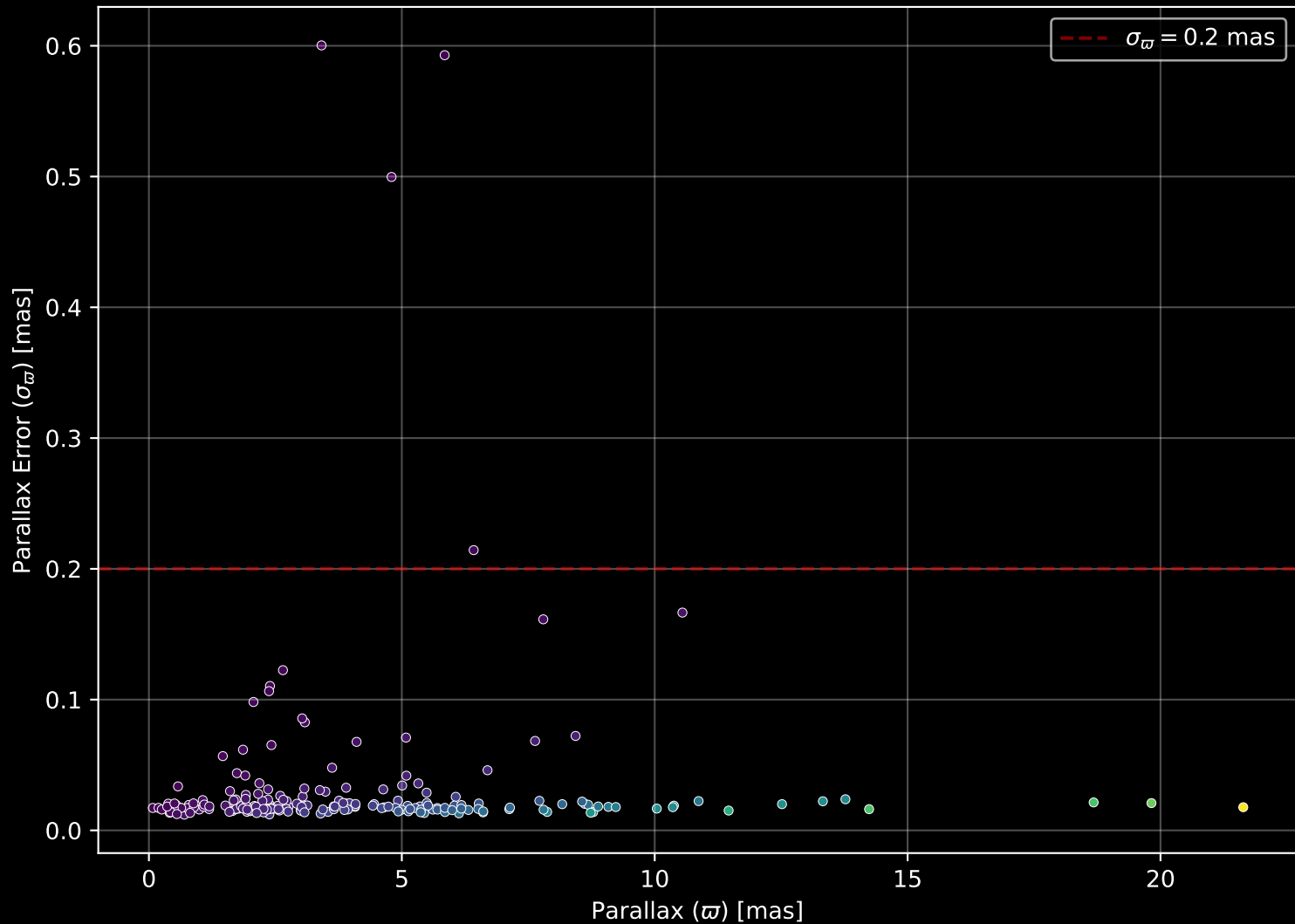
APOGEE DR17 Field: [K2_C12_077-57_btx] Parallax Quality (n= 200)
