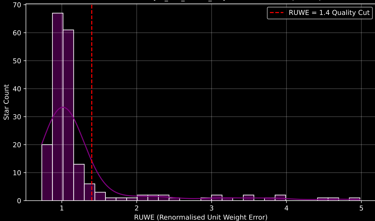
GAPOGEE DR17 Field [K2_C12_077-57_btx] RUWE Distribution (n= 192)
